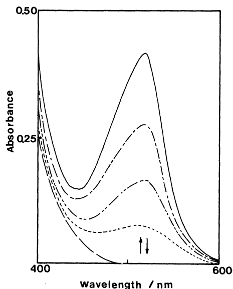
Fig. 3. Temperature effect on the absorption spectrum of the radical for 1 . The concentration of the radical is 2.4 \times 10^{-4} \text{ mol dm}^{-3} . (a) —, 25°C; (b) ---, 10°C; (c) — · —, -5°C; (d) · · · · ·, -20°C; (e) — — —, -50°C. These changes are reversible.
